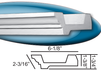
Bristol C305 (rigid)
