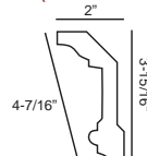
Camden C321 (rigid) FC321 (flexible**)
