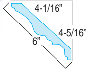
OUTSIDE CORNER WPC-124-OC
