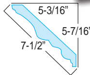
OUTSIDE CORNER WPC-127-OC
