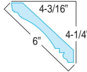
OUTSIDE CORNER WPC-121-OC
