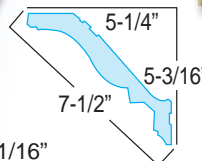
OUTSIDE CORNER WPC-130-OC
