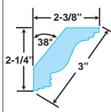
3" CROWN MOULDING PROFILE
