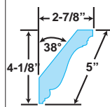
5" CROWN MOULDING PROFILE
