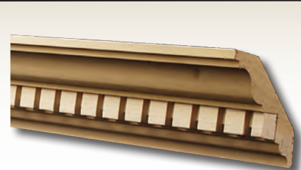
Crown 3/4" x 3-3/4" 2-1/2" approx. proj. 7/8" design repeat ADM455-POP
